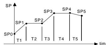
Fig. 1 - Example of a complete ramp and soak profile
