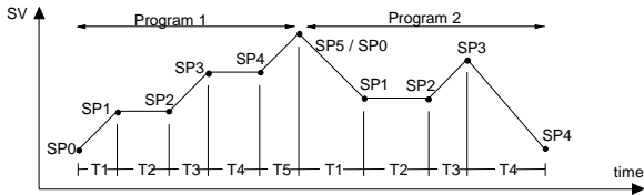
Fig. 3 - Example of two linked programs
